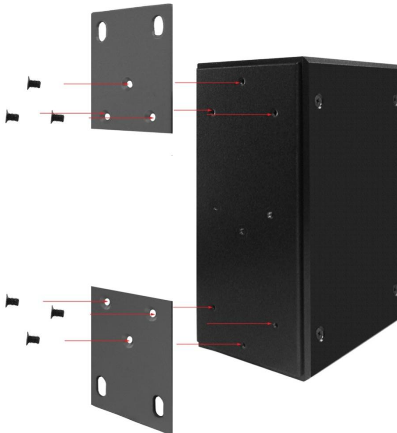
Figure-13: Wall-Mount Bracket Installation
