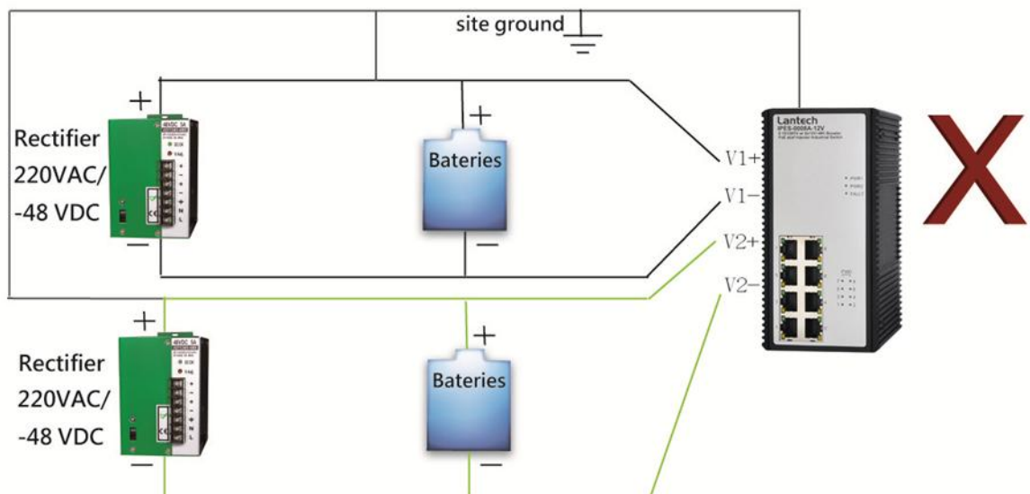
Dual battery solution- 2 negative power input (different power souce)
