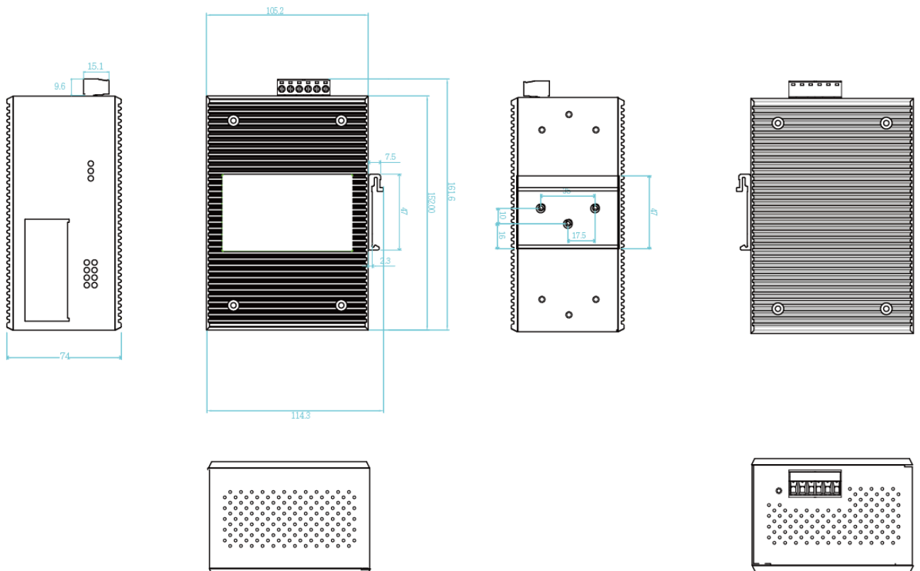
Figure-1: Mechanical Dimensions
