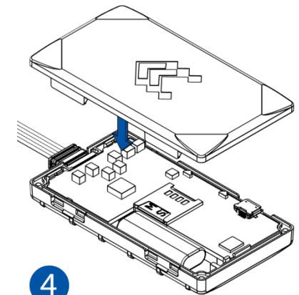
4 Figure 7 Attaching cover back
