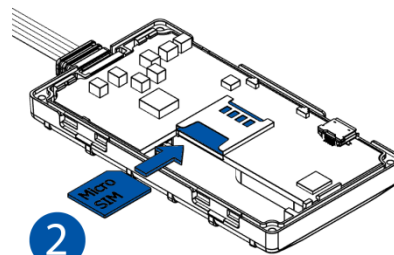
2 Figure 5 Micro-SIM card insert
