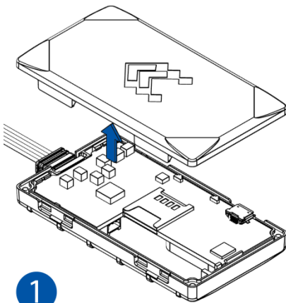
1 Figure 4 Cover removal
