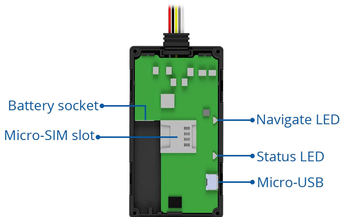
Figure 1 FMB920 device view
