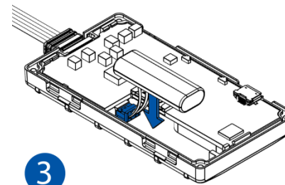
3 Figure 6 Battery connection
